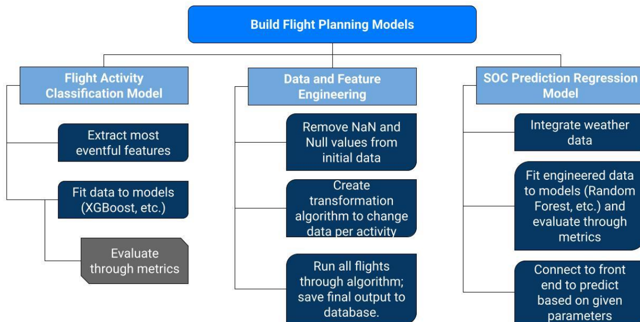
Figure 6: Diagram for both Machine Learning and DSS Model Needs
