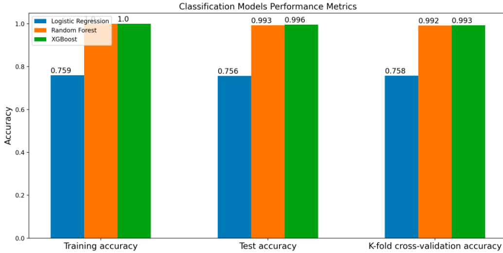
Figure 24: Classification Model Performance Metrics
