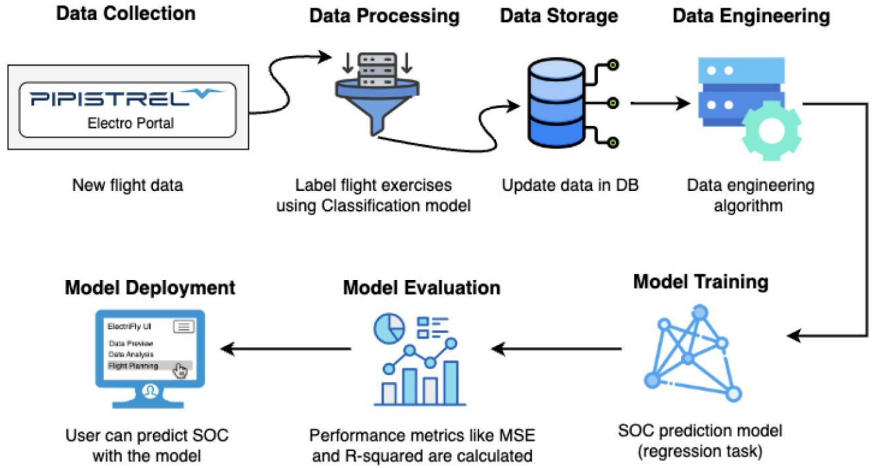
Figure 13: ML Pipeline Diagram
