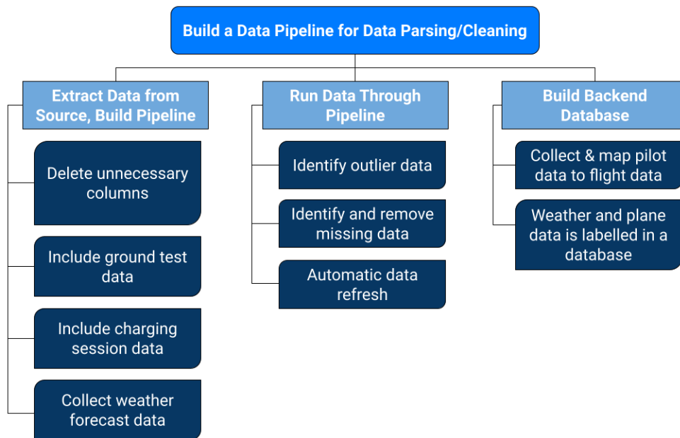
Figure 3: Diagram for both data pipeline
