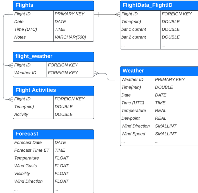
Figure 14: Database Schema
